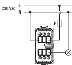
1-point light control
