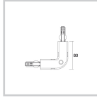
7805-00-W20/30/31 L joint
