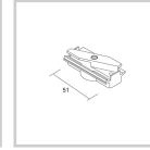
7825-00-30/31/52 Mechanical adapter
