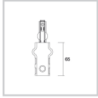
7802-00-W20/30/31 Live-end connector
